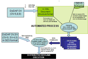
Figure 3: Process Methodology showing how automated modeling using XML can provide M&S to DoDAF documents
